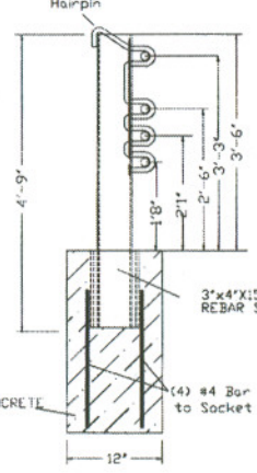
Line Post (Socketed)
