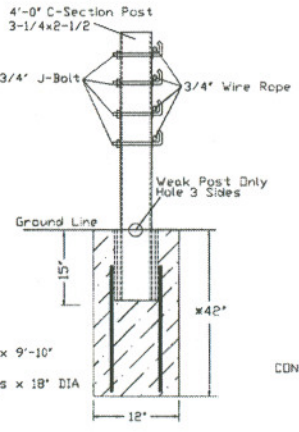
Terminal Post
