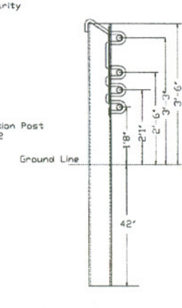
Line Post (Driven)
