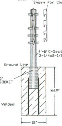
Line Post (Socketed)
